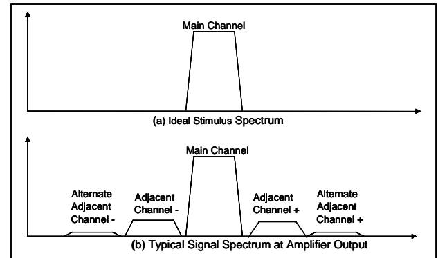
Fig. 2. Signal Spectrum Patterns
