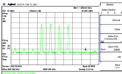
Fig. 6. GSM spectrum after cancellation
