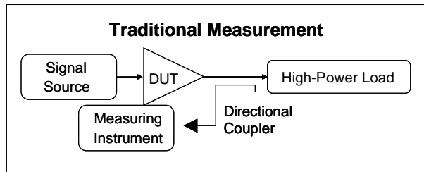
Fig. 1. High-Power Amplifier Measurement Setup
