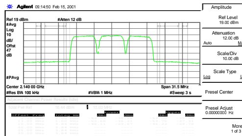
Fig. 9. Output power reduced 1-dB, ACP reduced at least 7 -dB
