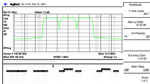
Fig. 7. W-CDMA with 3 carriers prior to cancellation
