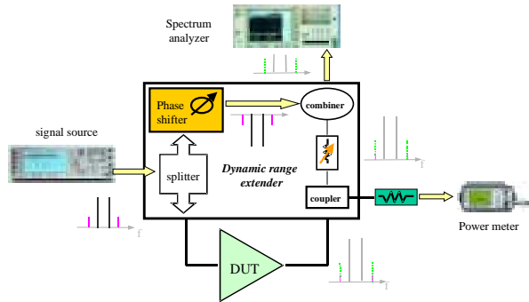
Fig. 3. Proposed Measurement System
